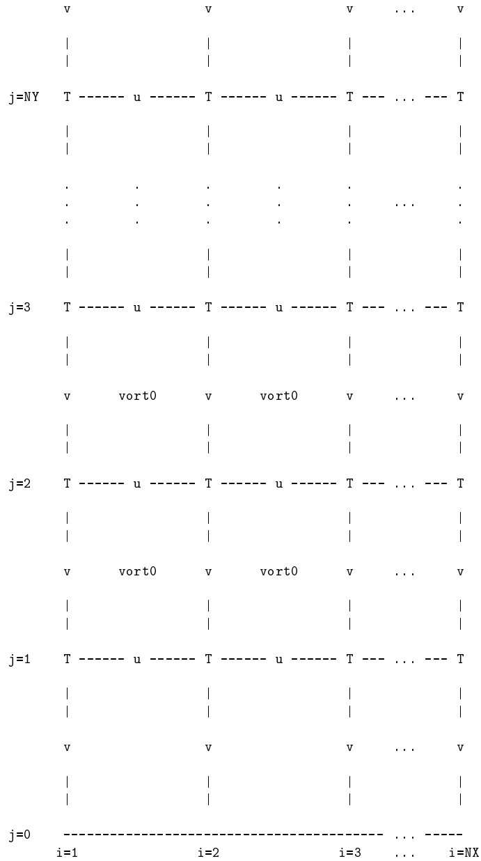
Figure 2.1: QTCM1 staggered C-grid. Note that j = 0 only exists for v and variables dependent on v . See text in Section 2.3.1 for details.
