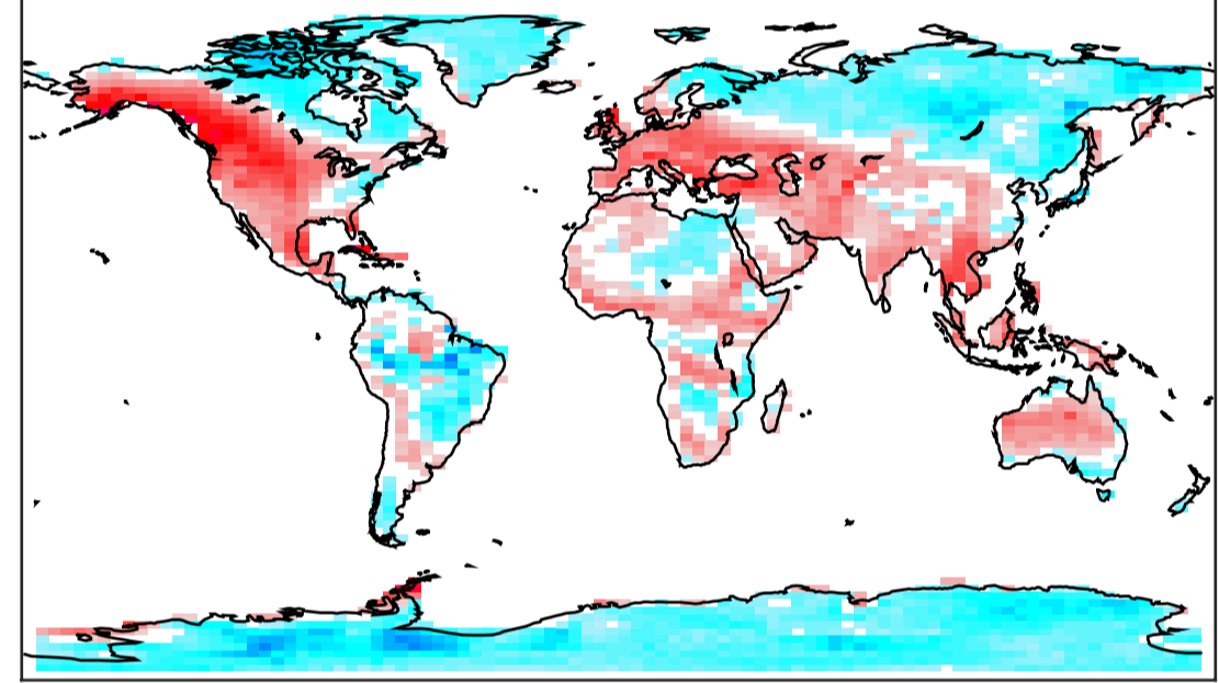
MIROC4h tasa djf thresh exceeds 79-05
