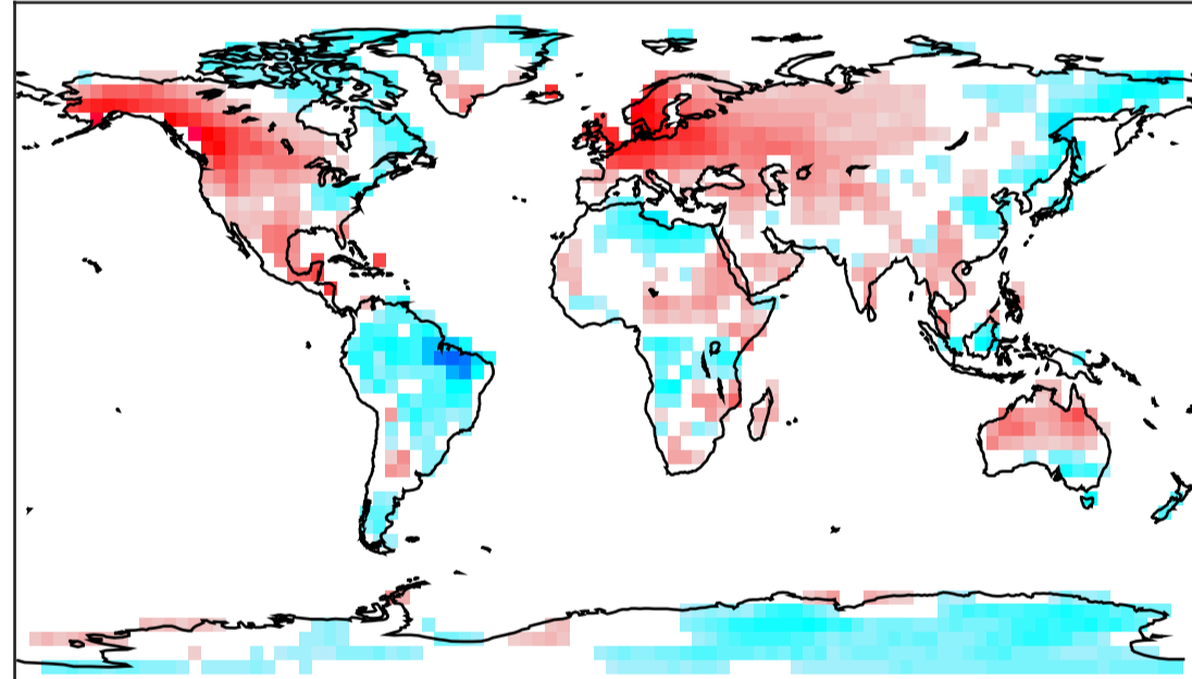
CMCC-CM tasa djf thresh exceeds 79-05
