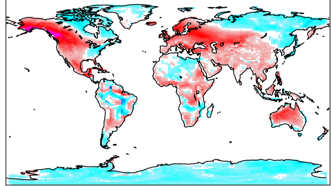
IPSL-CM5B-LR tasa djf thresh exceeds 79-05
