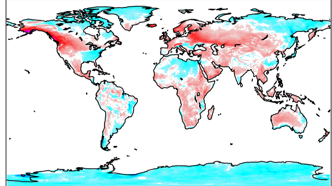
MIROC-ESM tasa djf thresh exceeds 79-05
