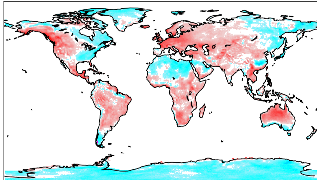
CMCC-CMS tasa djf thresh exceeds 79-05
