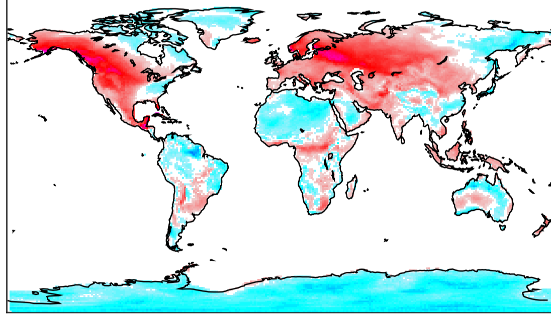
CESM1-CAM5 tasa djf thresh exceeds 79-05
