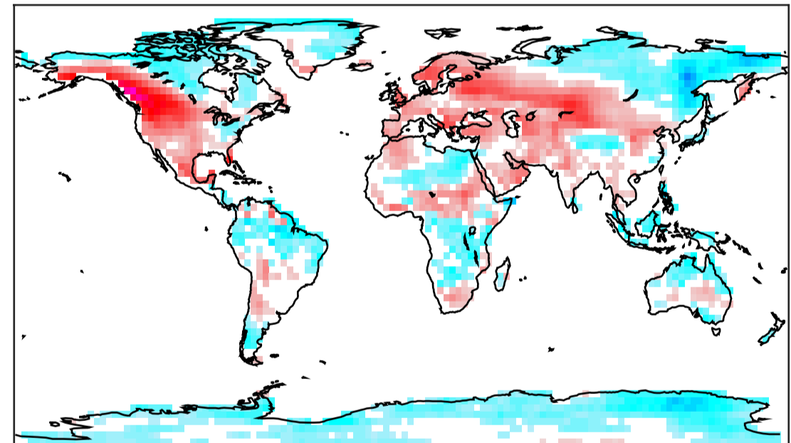
MIROC5 tasa djf thresh exceeds 79-05
