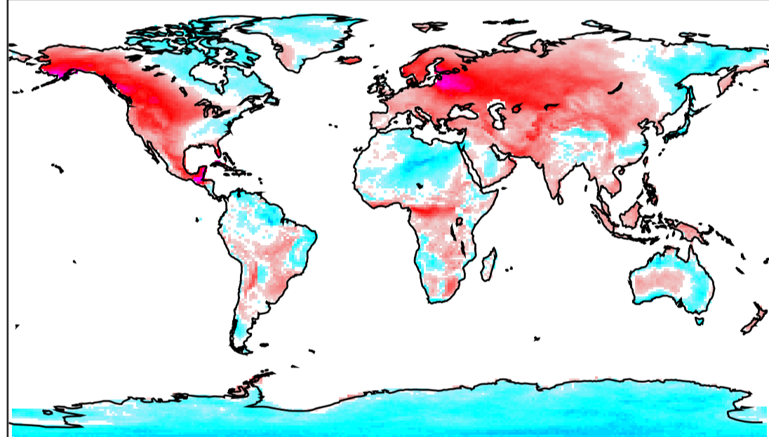
CMCC-CESM tasa jja thresh exceeds 79-05
