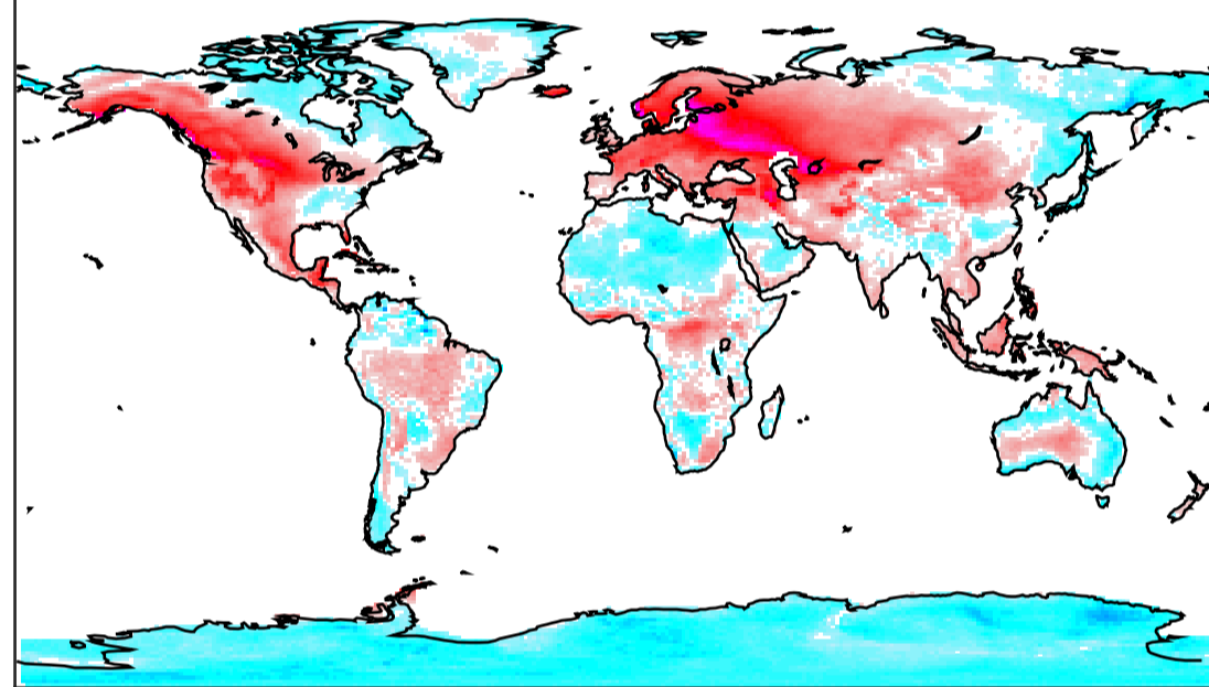
CESM1-FASTCHEM tasa djf thresh exceeds 79-05
