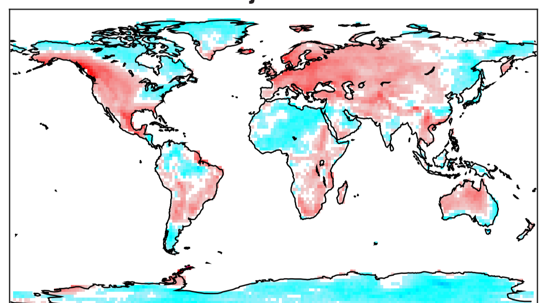
MPI-ESM-MR tasa jja thresh exceeds 79-05
