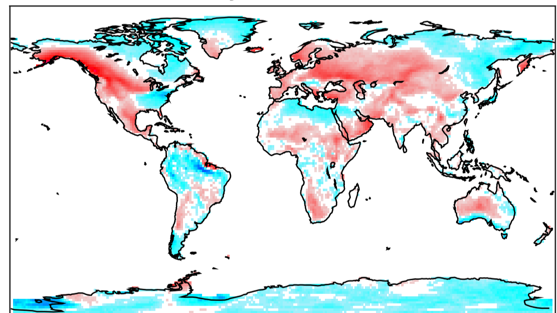
MPI-ESM-LR tasa djf thresh exceeds 79-05
