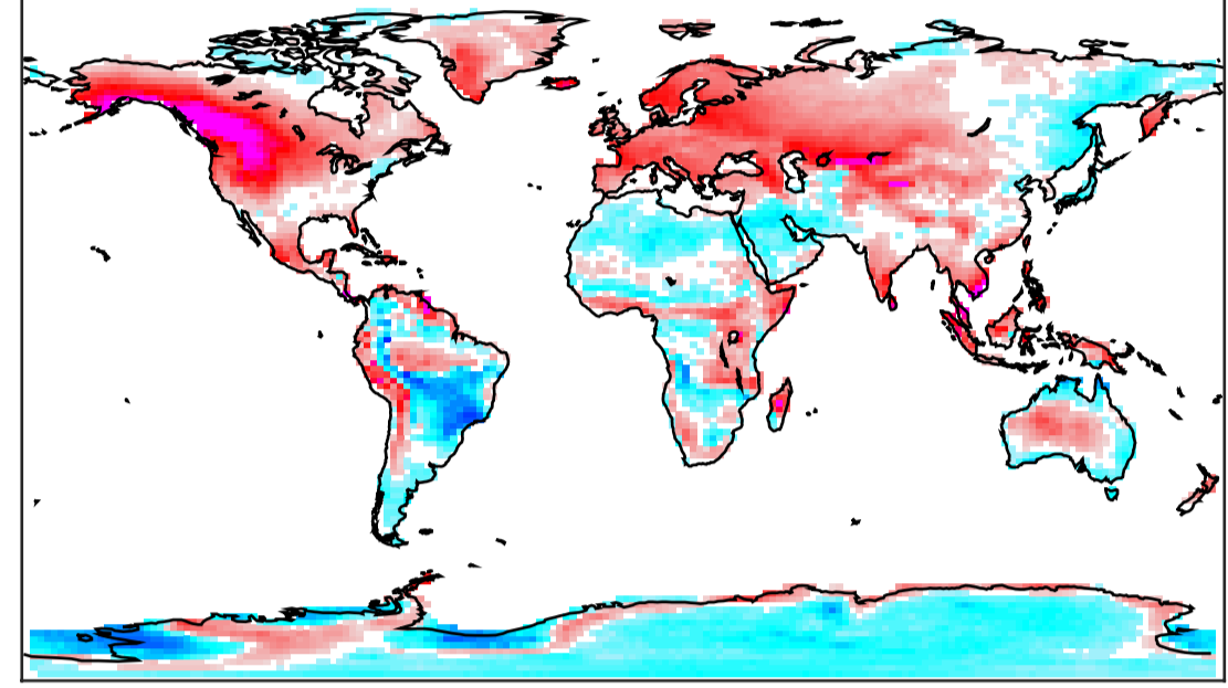
IPSL-CM5A-LR tasa djf thresh exceeds 79-05
