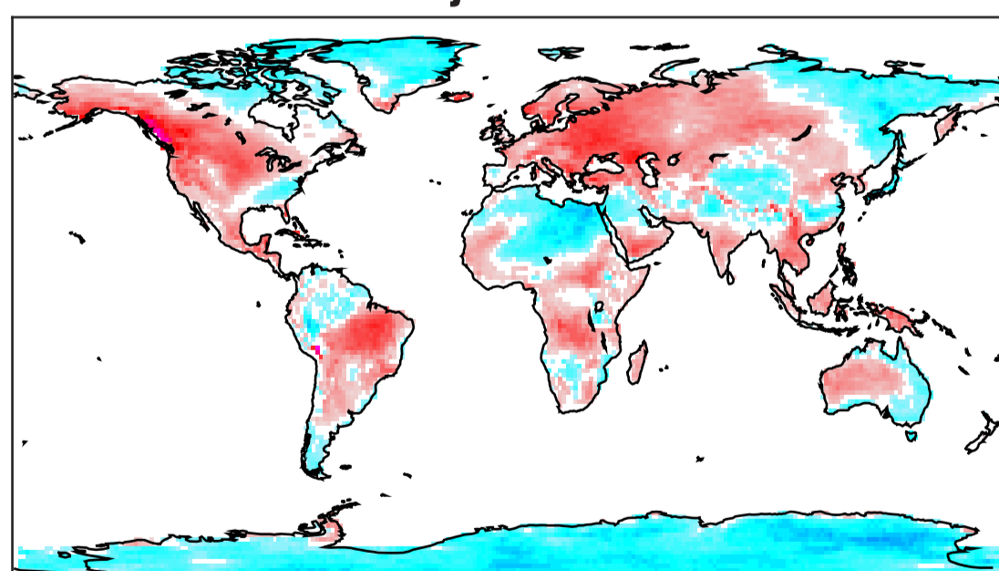
CSIRO-Mk3-6-0 tasa djf thresh exceeds 79-05
