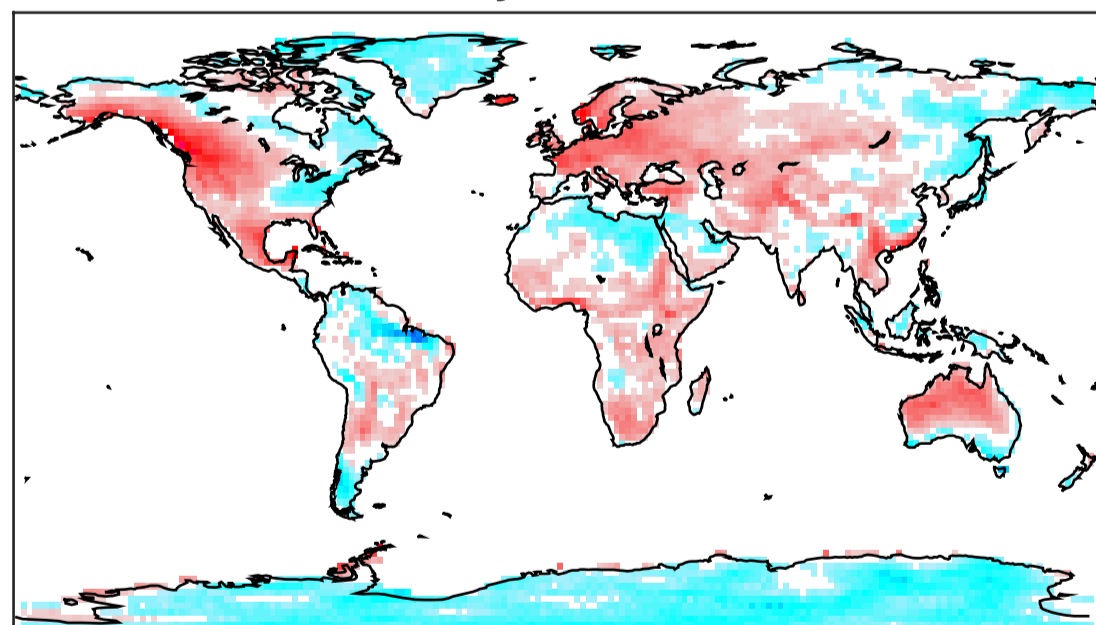
CNRM-CM5 tasa djf thresh exceeds 79-05
