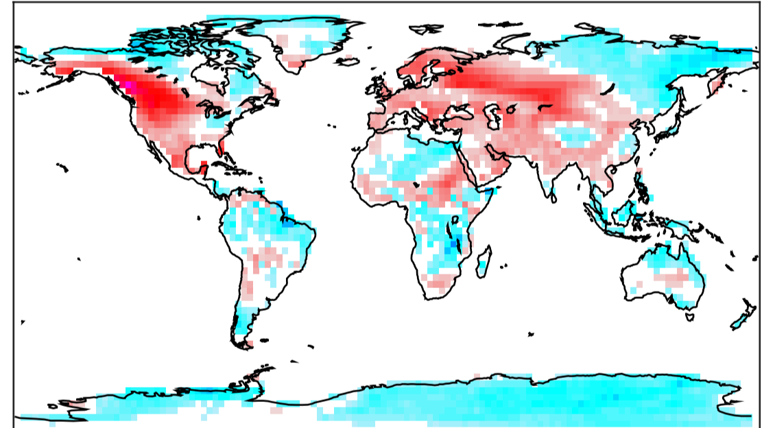
MIROC-ESM-CHEM tasa djf thresh exceeds 79-05
