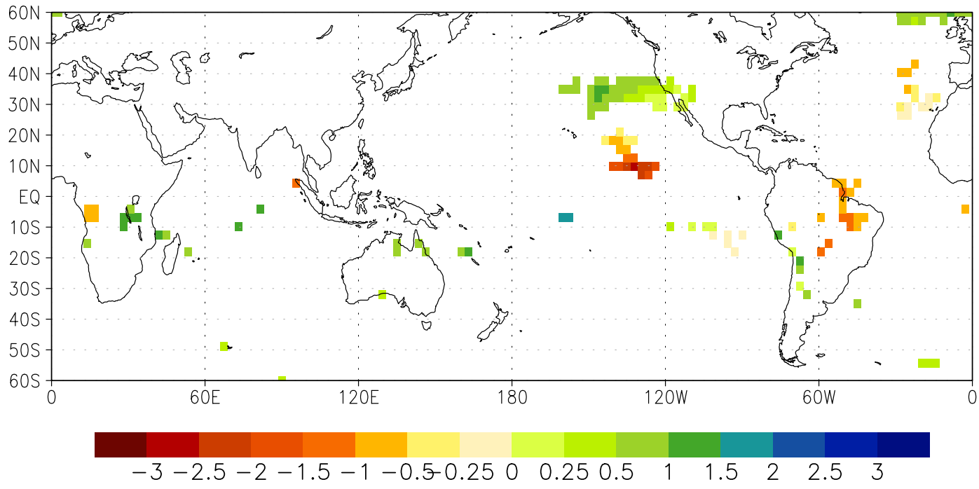
CanESM2 DJF Pra(76-05) wrt 1850-79 (95%)
