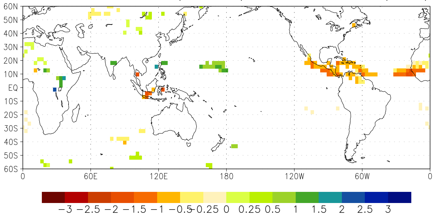
CanESM2 JJA Pra(76-05) wrt 1850-79 (95%)
