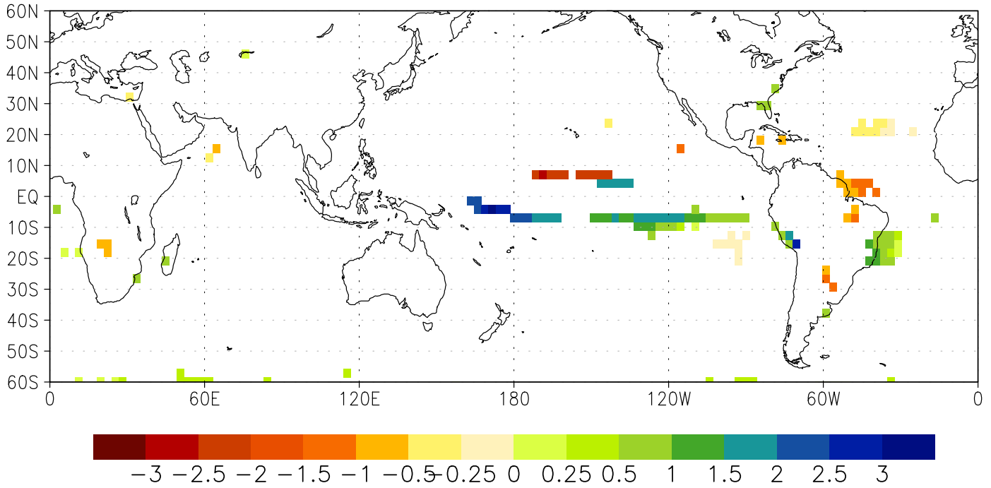
CanESM esmhist DJF Pra(76-05) wrt 1850-79 (95%)
