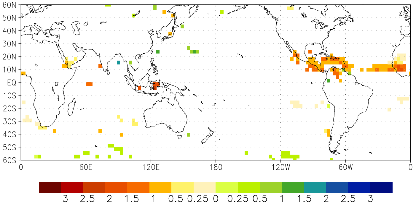
CanESM esmhist JJA Pra(76-05) wrt 1850-79 (95%)
