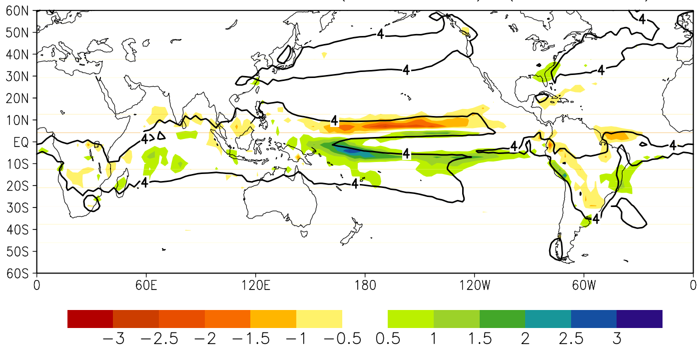
cccmaESM DJF Pa(1976-05) (1850-79)
