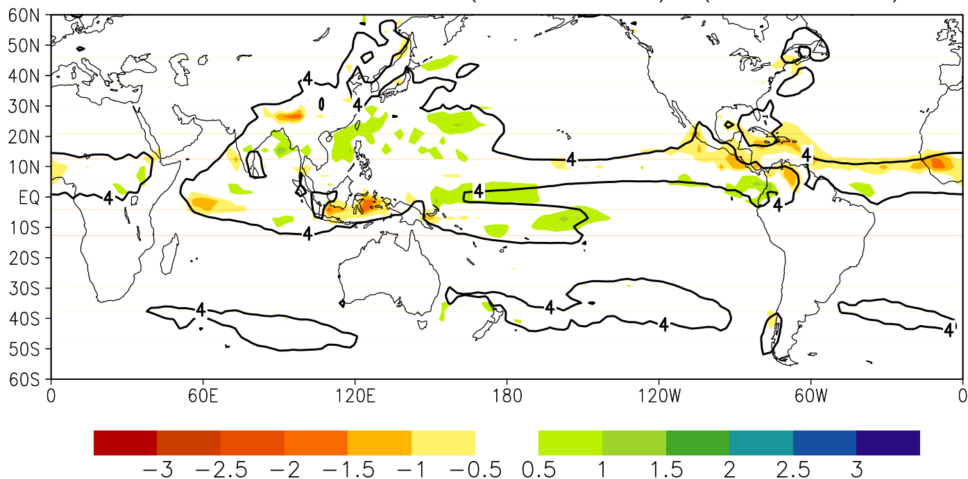
cccmaESM JJA Pa(1976-05) (1850-79)
