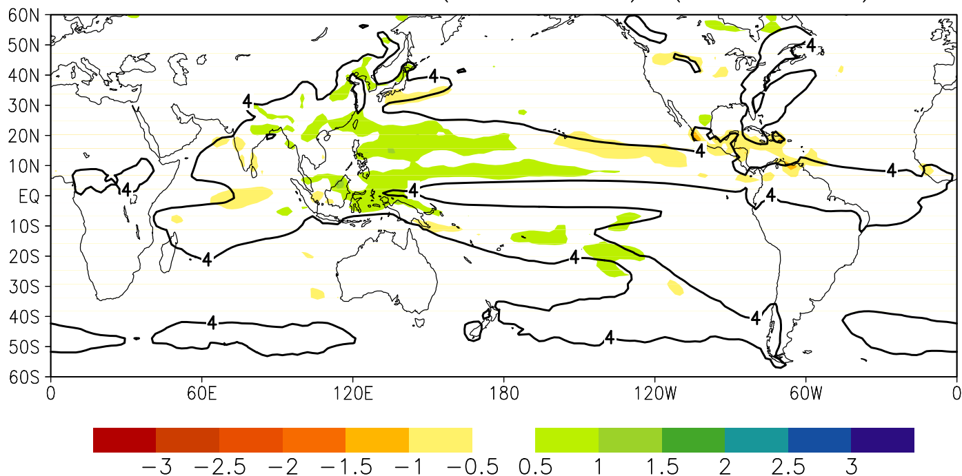
inmcm4 JJA Pa(1976-05) (1850-79)
