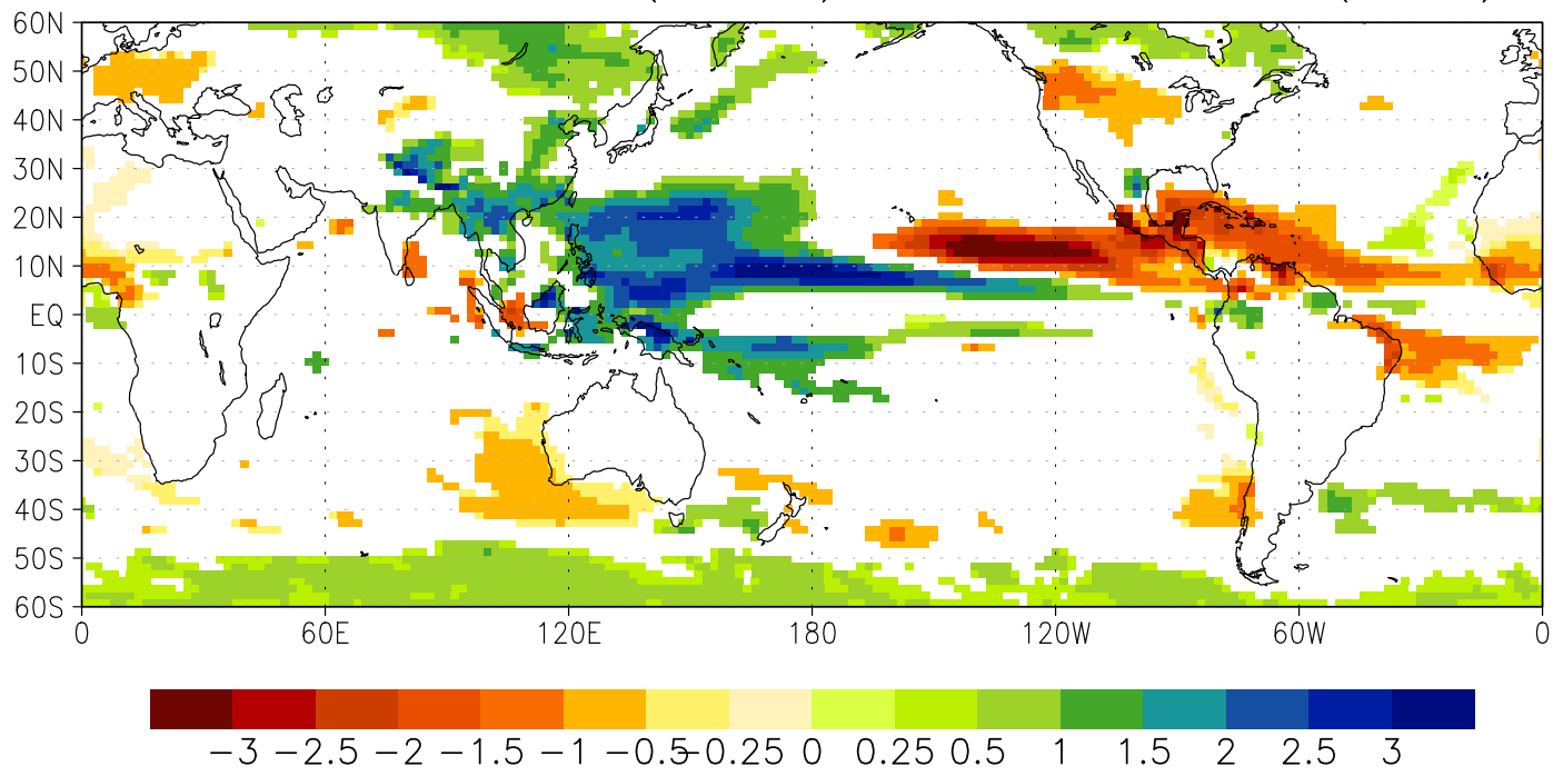
inmcm4 JJA Pra(2085) wrt 1850-79 (95%)
