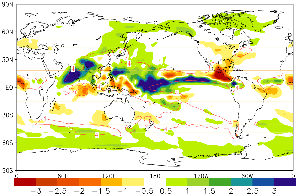
bcc esmrcp8.5 JJA Prec(2070-99) (1850-79)
