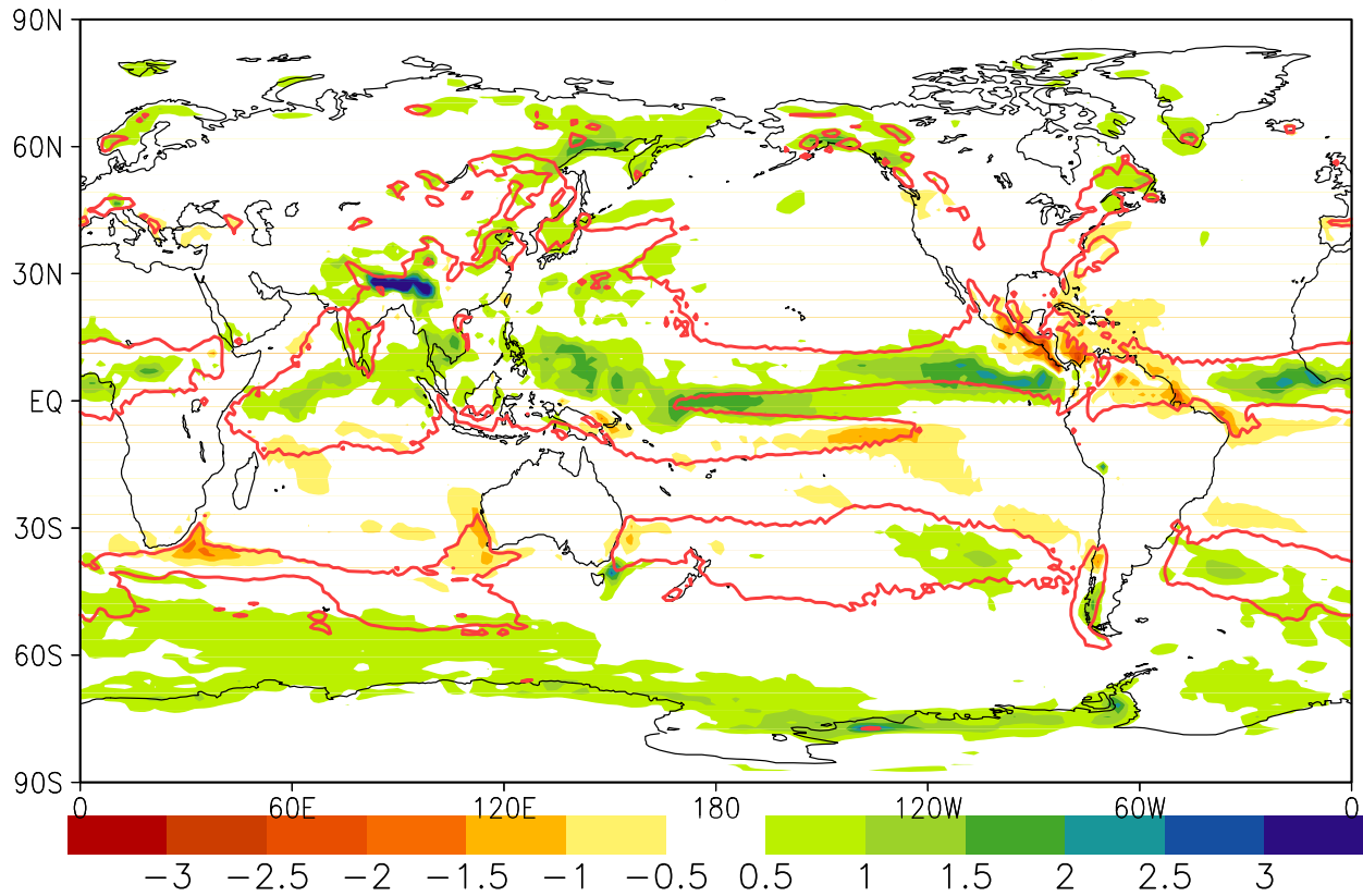
cnrm rcp8.5 JJA Prec(2070-99) (1850-79)
