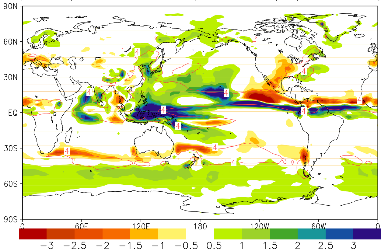
ipsl rcp8.5 JJA Prec(2070-99) (1850-79)
