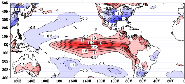
WARM-COLD(sstn34.abs.gt.0.8) DJF: INMCM4 cmip5(amip) Ts (83 87 92 95 98 03) - (84 85 89 96 99 00 01)
