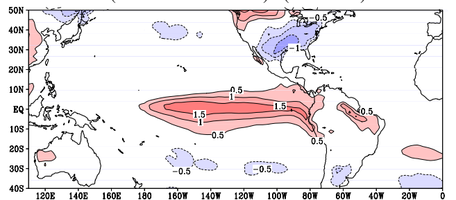
ENSO-Clim DJF: NORESM1cmip5(amip) Ts (83 87 88 92 95 98 03) - (79-05clim)
