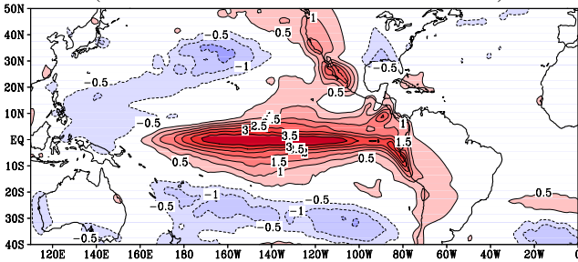
WARM-COLD(sstn34.abs.gt.0.79 DJF: CNRM cmip5(amip) Ts (83 87 88 92 95 98 03) - (84 85 89 96 99 00 01)
