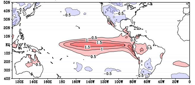
(a) ENSO-Clim DJF: HadGEM-a cmip5(amip) Pr (83 87 92 95 98) - (79-05clim)
