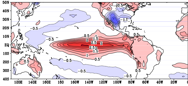
WARM-COLD(sstn34.abs.gt.0.79) DJF: NORESM1cmip5(amip) Ts (83 87 88 92 95 98 03) - (84 85 86 89 96 99 00 01)
