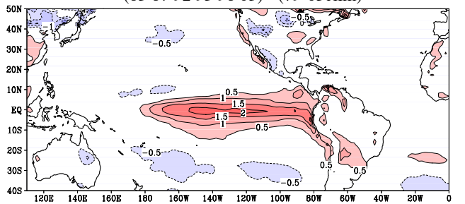
ENSO-Clim DJF: IPSL cmip5(amip) Ts (83 87 88 92 95 98 03) - (79-05clim)
