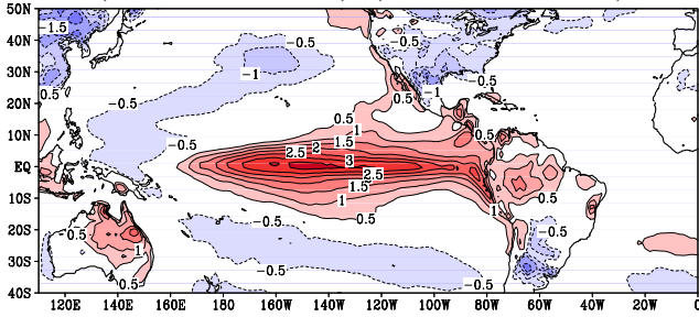
WARM-COLD(sstn34.abs.gt.0.81) DJF: HadGEM-a cmip5(amip) (83 87 92 95 98) - (84 85 87 96 99 00 01)
