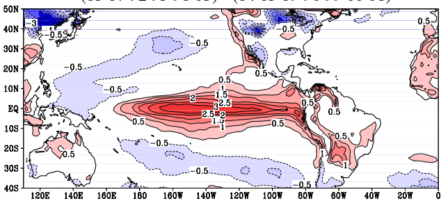
WARM-COLD(sstn34.abs.gt.0.79) DJF: IPSL cmip5(amip) Ts (83 87 88 92 95 98 03) - (84 85 89 96 99 00 01)
