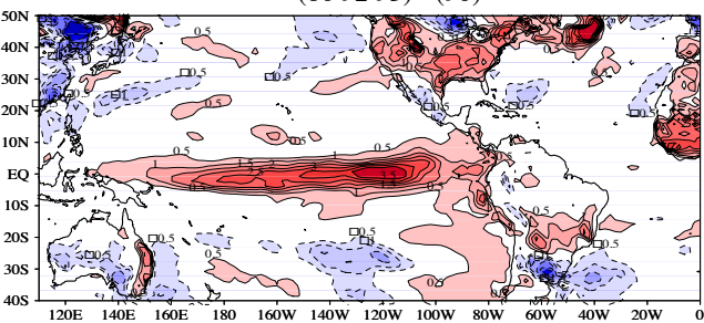
WARM-COLD(abs.gt.1.2) DJF: GISS-H cmp5(hist) Skin (81 84 91) - (85 92 03)
