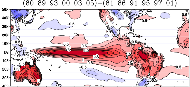
) WARM-COLD(abs.gt.1.01) DJF: CanESM cmp5(esmhist) (80 89 93 00 03 05) - (81 86 91 95 97 01)
