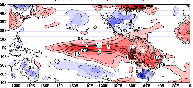
(a) WARM-COLD(abs.gt.0.86) DJF: CNRM cmp5(hist) Pr (82 90 91 94 98 00) - (81 89 92 95 96 99 01 03)
