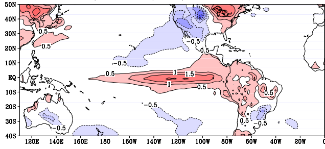
(a) ENSO-Clim DJF: GISS-R cmp5(hist) Skin T (90 99 02) - (79-05clim)
