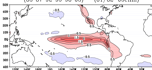
(a) ENSO-Clim DJF: REYNOLDS SST (83 87 92 95 98 03) - (81/82-05clim)
