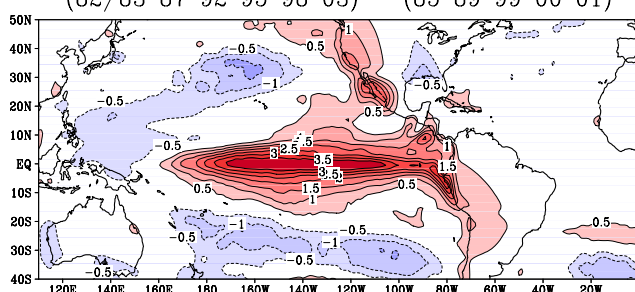
(a) WARM-COLD(abs.gt.0.85) DJF: REYNOLDS SST (82/83 87 92 95 98 03) - (85 89 99 00 01)
