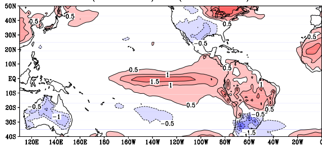
(a) ENSO-Clim DJF: CNRM cmp5(hist) Pr (82 90 91 94 98 00) - (79-05clim)
