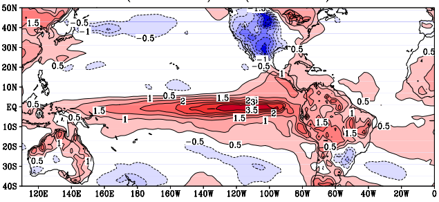
WARM-COLD(abs.gt.0.74) DJF: GISS-R cmp5(hist) Skin (90 99 02) - (92 94 97)
