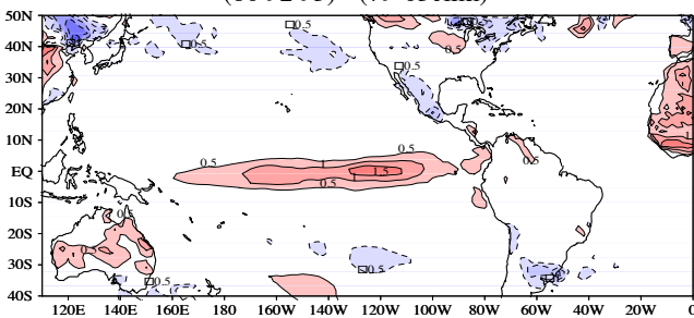
(a) ENSO-Clim DJF: GISS-H cmp5(hist) Skin T (81 84 91) - (79-05clim)
