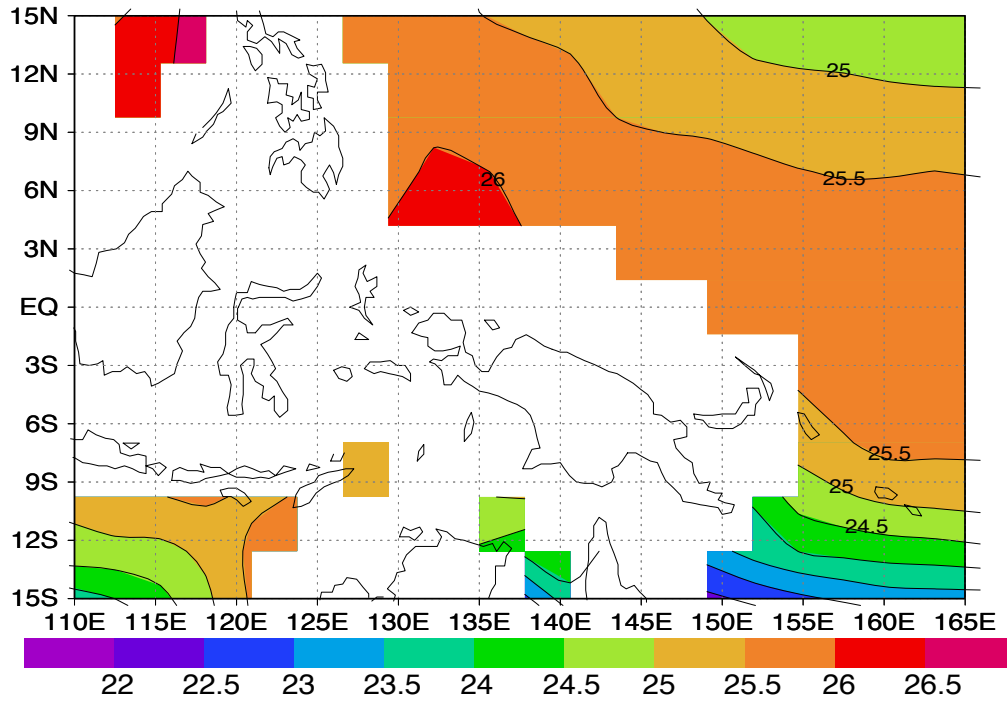
T 1000 ccsm3 JJA 0k
