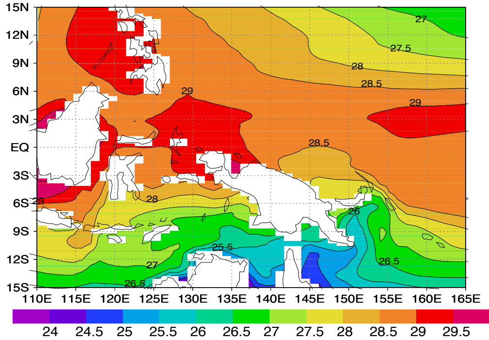
sst ccsm3 JJA 0k
