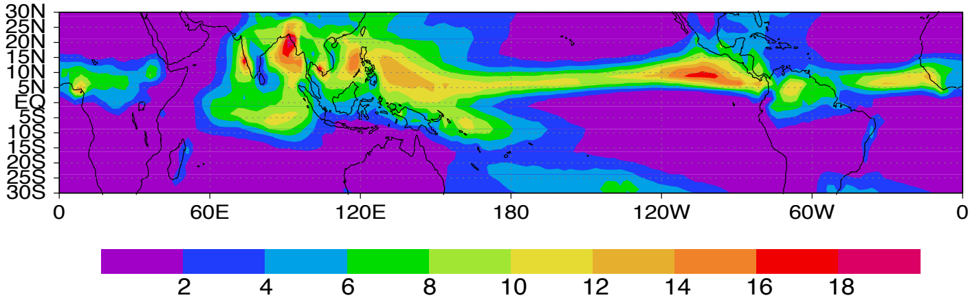
prec CMAP JJA 1/79-9/09
