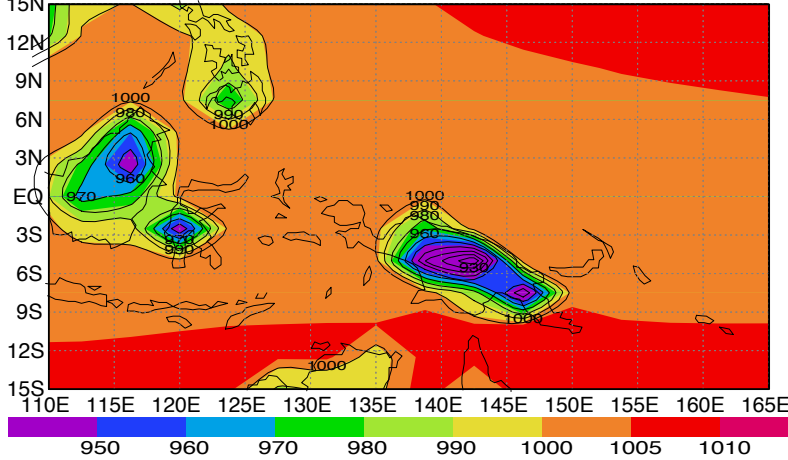
sfc pres miroc JJA 0k
