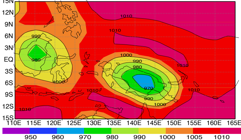
sfc pres miroc JJA 0k
