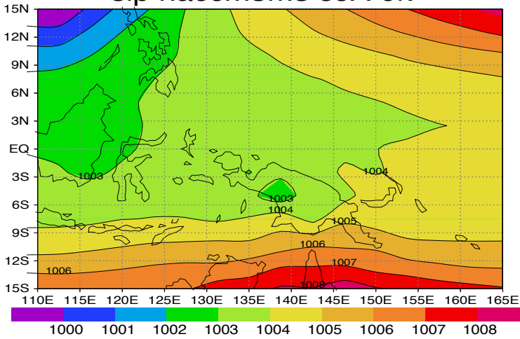
slp miroc JJA 0k
