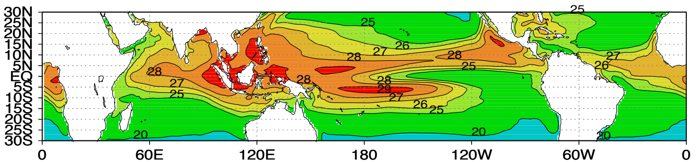
sst ccsm3 JJA 0k
