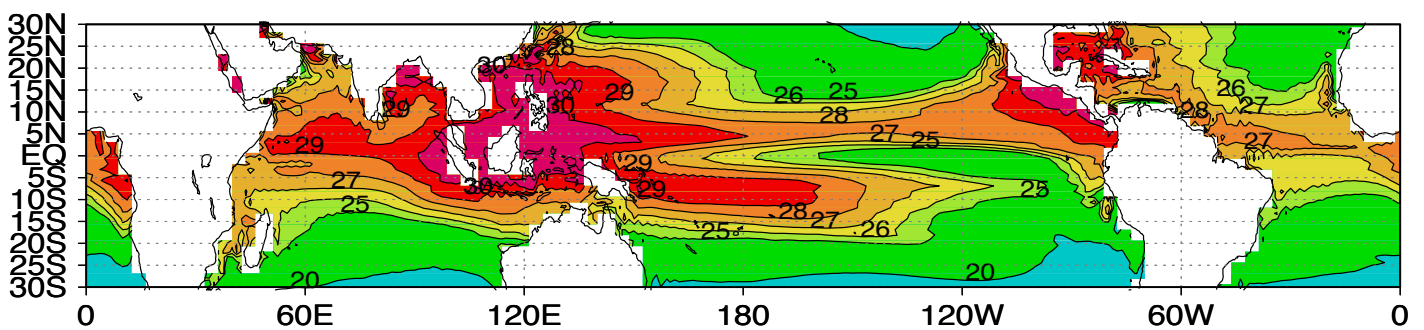
sst hadcm3m3 JJA 0k
