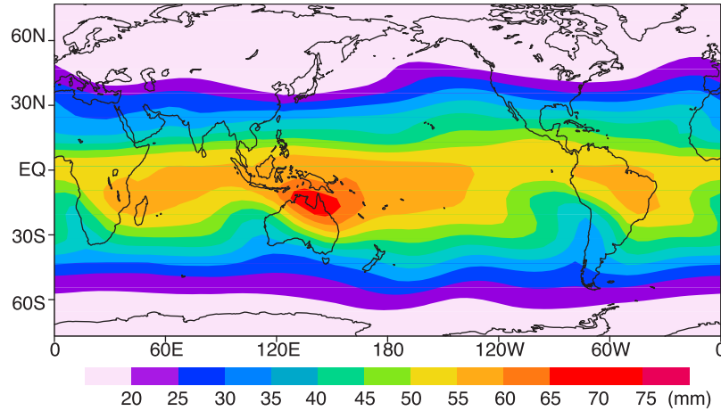
Figure 4. Comparison of DJF CWV from (a) the NCEP Reanalysis 2 and QTCM2 at (b) high resolution and (c) low resolution. Units are in mm.
