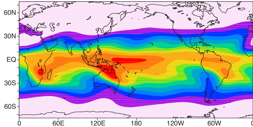
c) QTCM2 (lores) DJF 1000-150mb CWV
