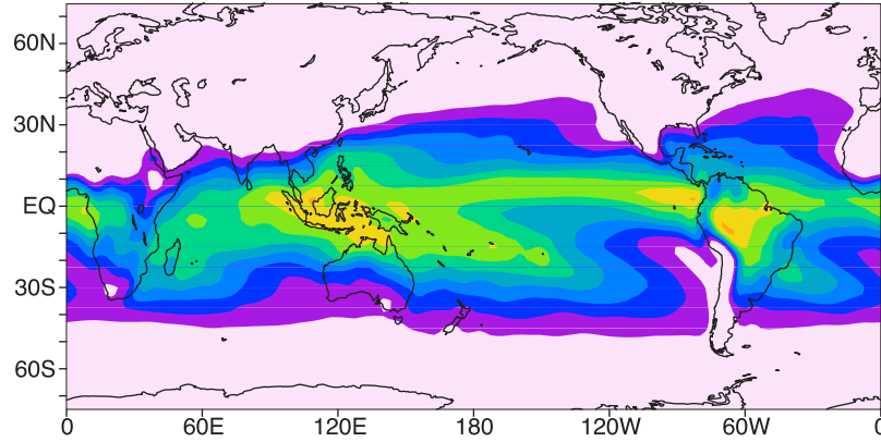
b) QTCM2 (hires) DJF 1000-150mb CWV
