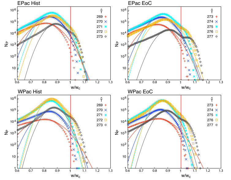
FIG. 6. Similar to Fig. 2 with the left column for the historical and right for the EoC for tropical eastern and western Pacific (top and bottom rows, respectively). As in Fig. 2, the procedure tends to collapse in occurrence statistics of rescaled column water vapor for precipitating points for different values of \hat{T} confirming that the leading effects are controlled by the critical values.
