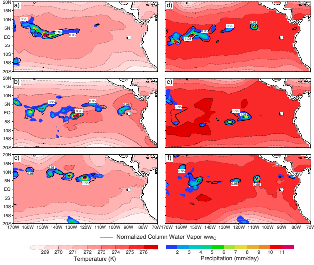
FIG. 7. Instantaneous snapshots of precipitation, \hat{T} , and rescaled CWV ( w/w_c ; with w_c linearly interpolated as a function of \hat{T} for each of the grid points), for the historical (a-c), and EoC (d-f), in chronological order. Dotted lines with shading are for \hat{T} , solid lines with shading for precipitation, and solid black contours for w/w_c . The snapshots have been chosen from the tail of the distribution for the higher \hat{T} from the historical and EoC, such that each of them has at least one grid point with w/w_c near 1.1, representing the extremes.
