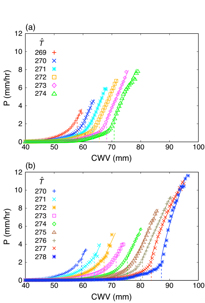
FIG. 3. Precipitation pickup for 1 degree CCSM4 over the tropical eastern Pacific, similar to Fig. 1a: (a) Historical (1981-2000), and (b) End-of-century (EoC; 2081-2100) for the Representative Concentration Pathway 8.5 (RCP8.5) scenario.
