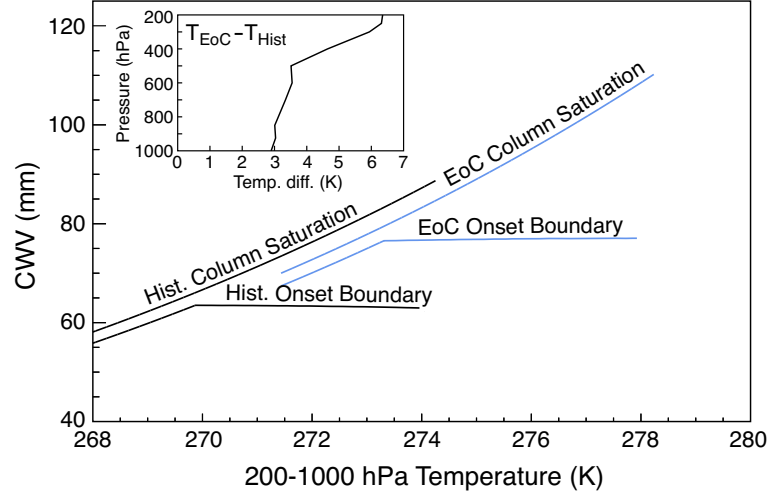
FIG. 8. Precipitation onset boundary, similar to that shown in Figs. 1c and 5, but for a simplified prototype using idealized perturbations to Nauru profiles. Contours of 100 J/kg entraining CAPE computed by a one-dimensional entraining plume model, or free tropospheric saturation (seen at lower \hat{T} -values, see text), are shown as a measure of the onset boundary of precipitation (by conditional instability or large-scale saturation) for the historical and EoC. The model and the procedure are similar to that discussed in SNHN12. For the historical computations vertically constant temperature perturbations of 0.2 K are applied to the Nauru mean state conditioned on high values of CWV representative of deep convective cases, whereas for the EoC, similar perturbations are applied to the conditioned temperature profile shifted by the CCSM4 temperature anomaly profile over Nauru for the EoC (shown in the inset). The corresponding column saturation curves are shown for comparison.
