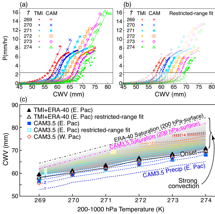
FIG. 1. (a) Conditional average precipitation as a function of CWV for different bins of \hat{T} over the tropical eastern Pacific from TMI using the ERA-40 temperature profiles and a 0.5 degree resolution version of CAM3.5. Power-law fit lines (solid curves, see text) are shown above the critical value w_c , where precipitation undergoes a rapid increase (vertical dashed lines starting at P=2.5 mm/hr connect the fit curves to the estimates of w_c on the x-axis). A power-law exponent of 0.23 is fit for the TMI retrieval whereas for the model it is 1. (b) As in (a) but for a linear fit over a restricted range. (c) The critical column water vapor w_c from retrievals (TMI) and model (CAM3.5) as a function of bulk tropospheric temperature \hat{T} . Critical values from two fitting methods, corresponding to (a) and (b), are shown for eastern Pacific TMI and CAM3.5. Western Pacific values from CAM 3.5 are shown for the first method. Contours of CAM3.5 conditional average precipitation are shown in background (dashed lines). Also shown for reference are the values for column saturation (dash-dotted) from both ERA-40 and CAM3.5.
