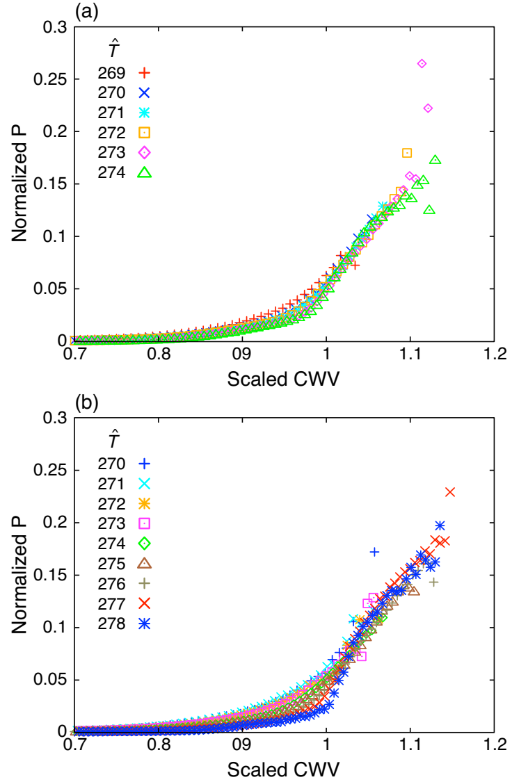
FIG. 4. Ensemble average precipitation over the tropical eastern Pacific as a function of column water vapor rescaled by the corresponding w_c for each of the \hat{T} bins at 1 K intervals: (a) Historical, and (b) EoC for RCP8.5 warming, showing the collapse of the curves over the range of \hat{T} .
