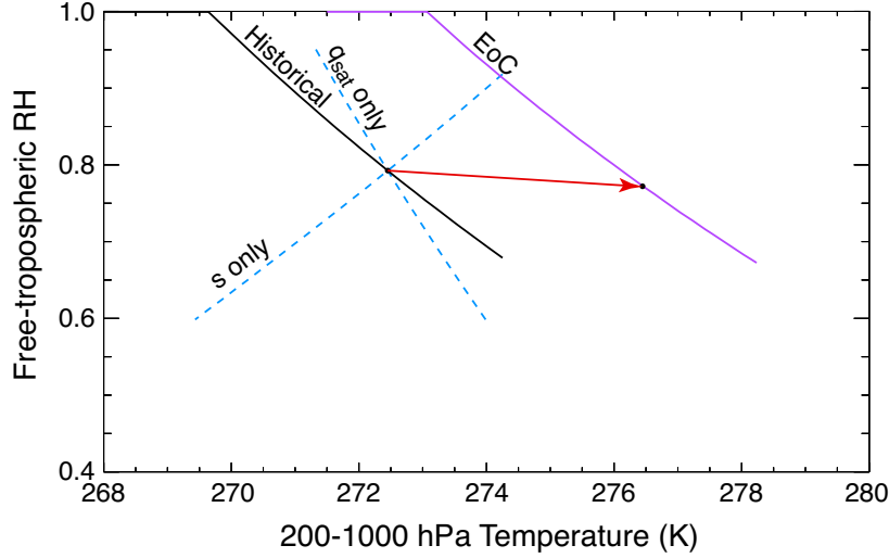
FIG. 9. Simplified prototype for the onset boundary for the present day (solid black curve marked historical) and global warming (solid purple curve marked EoC). These curves correspond to Fig. 8, except that the moisture axis is given in terms of free-tropospheric relative humidity. The red arrow indicates shift associated with global warming temperature change profile. Temperature changes along the historical and EoC curves have a different vertical profile (as in Fig. 8). Dashed lines for the historical case show calculations that examine the effects of temperature via dry static energy ‘s’ and ‘ q_{sat} ’ in the conditional instability calculation that defines the onset boundary.
