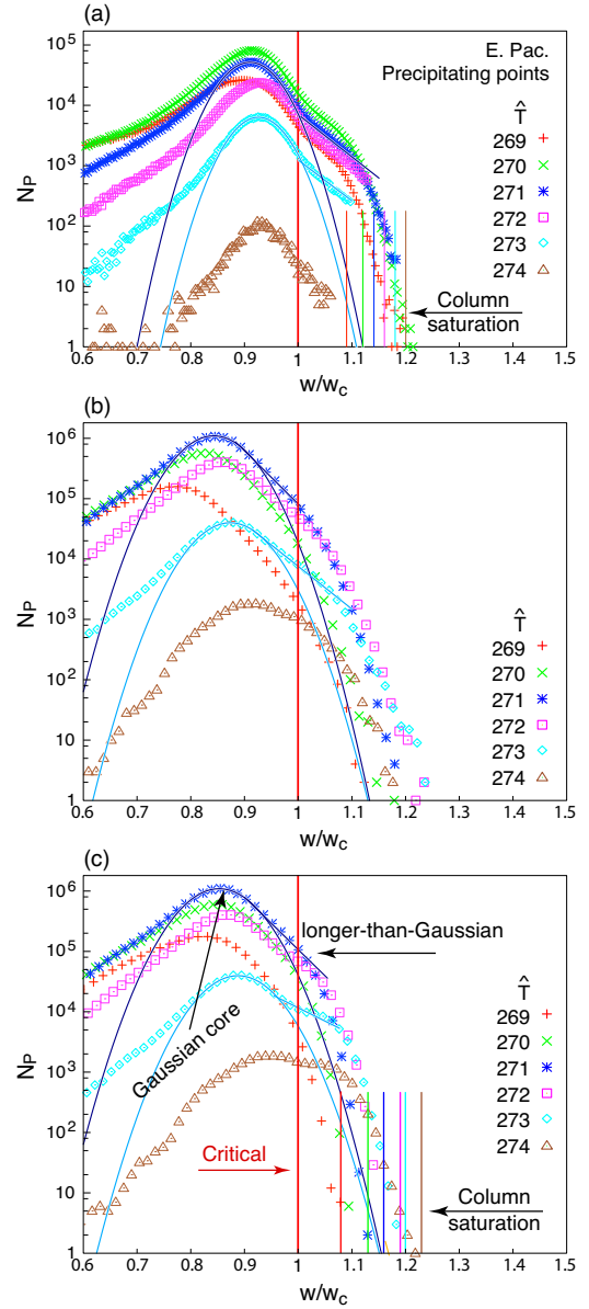
FIG. 2. Log-linear plot of the frequency of occurrence ( N_p ) of CWV rescaled by the corresponding onset threshold values w_c(\hat{T}) for precipitating points over the tropical eastern Pacific binned for \hat{T} values at 1 K intervals (curve shapes are the same as PDFs aside from a shift corresponding to a normalization constant). (a) TMI precipitation and column water vapor binned by ERA-40 temperatures, (b) 0.5 degree CAM3.5 precipitation and column water vapor binned by bulk tropospheric temperatures computed at a coarsened resolution of 2.5 degrees for a better comparison with panel (a), and (c) 0.5 degree CAM3.5 precipitation and column water vapor binned by bulk tropospheric temperatures computed at native model resolution. Gaussian fits (parabolas) to the core and exponential fits (straight lines) to the tail are shown for selected \hat{T} curves to aid comparison. Vertical bars indicate column saturation values corresponding to \hat{T} values of the same color.
