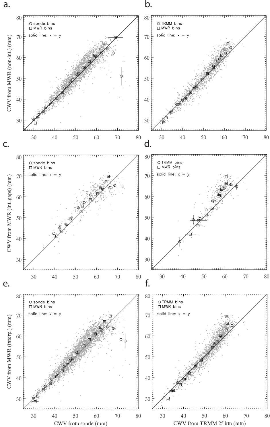
FIG. 3. Conditional averages and associated standard errors of column water vapor values for MWR vs. sondes and vs. TRMM (with scatter plots in background), for (a,b) non-gap-filled MWR data; (c,d) only the filled gaps in the MWR data; and (e,f) full interpolated MWR data. Conditional averages are performed (binned) on each variable in turn. Bins are 3 mm wide, and only bins with at least 5 counts are plotted.
