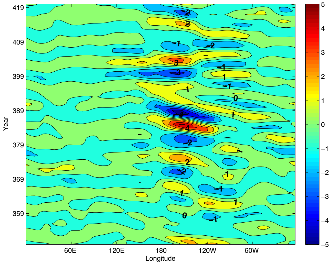
R30 SAT, bandpassed on 5–12 years, 72S, time vs longitude
