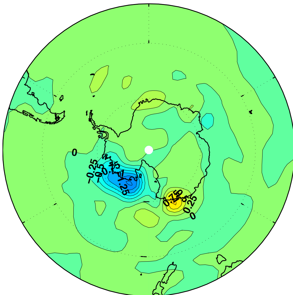
R30 SST, 32–64 years bandpass, Year 541
