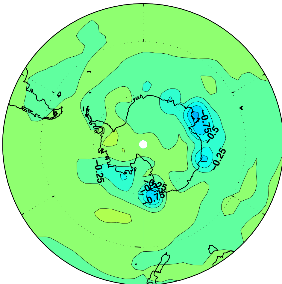
R30 SST, 32–64 years bandpass, Year 549
