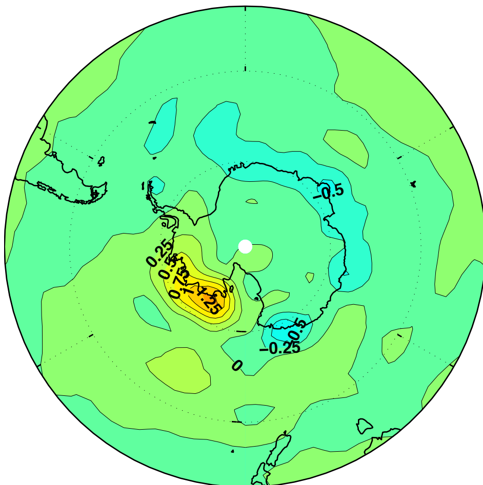
R30 SST, 32–64 years bandpass, Year 557
