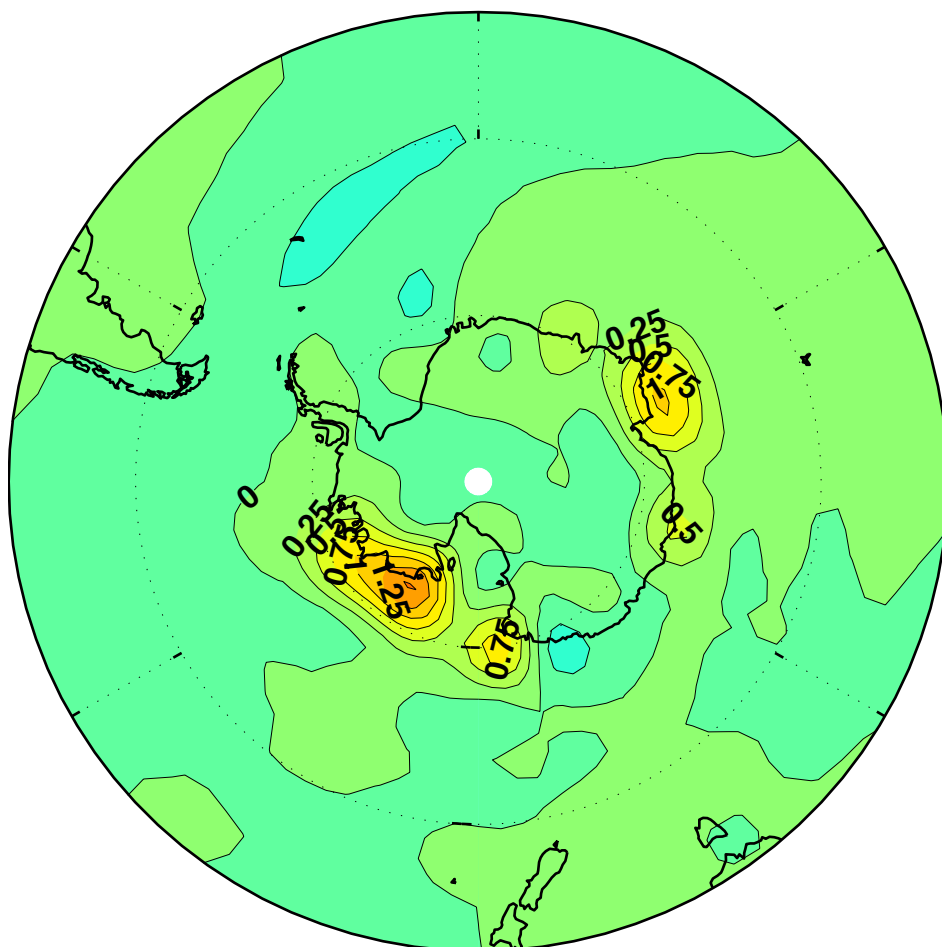
R30 SST, 32–64 years bandpass, Year 565
