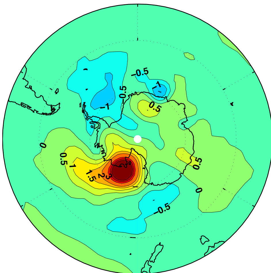
R30 SST, 5–12 years bandpass, Year 385
