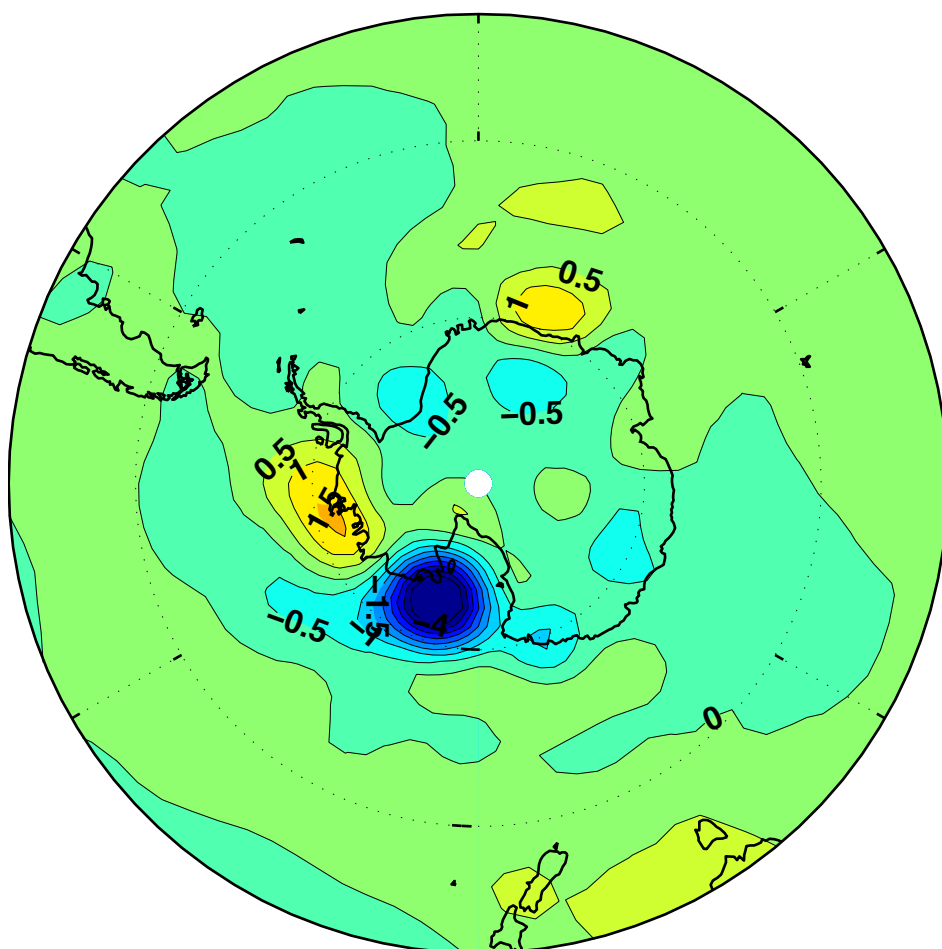
R30 SST, 5–12 years bandpass, Year 389
