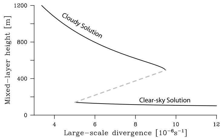
FIG. 4. A conceptual illustration for the MLM's multiple equilibria behavior, after Randall and Suarez (1984). Two solid lines are the stable solutions: cloudy and clear-sky. Dashed line is the unstable solution.
