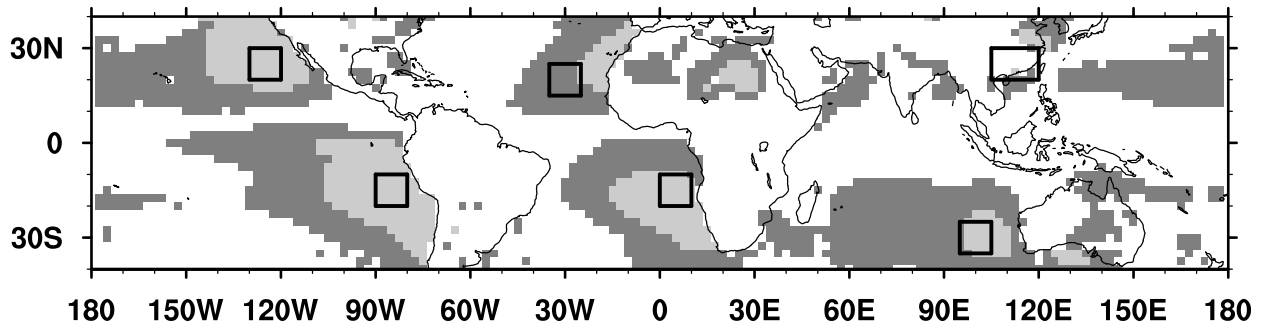
FIG. 2. Boxes show the subtropical stratocumulus regions from Klein and Hartmann (1993): California ( 20^{\circ} - 30^{\circ} N, 120^{\circ} - 130^{\circ} W), Canarian ( 15^{\circ} - 25^{\circ} N, 25^{\circ} - 35^{\circ} W), China ( 20^{\circ} - 30^{\circ} N, 105^{\circ} - 120^{\circ} E), Peruvian ( 10^{\circ} - 20^{\circ} S, 80^{\circ} - 90^{\circ} W), Namibia ( 10^{\circ} - 20^{\circ} S, 0^{\circ} - 10^{\circ} E), and Australia ( 25^{\circ} - 35^{\circ} S, 95^{\circ} - 105^{\circ} E). Shading denotes locations where the climatological (1987-2001) conditions are suggestive of low-cloud conditions: vertical motion in the mid- (500 hPa) and lower-troposphere (700 hPa) greater than 10 hPa/day in at least one season and the lower-tropospheric stability (LTS) based on ECMWF Reanalysis (ERA-40) data. Light shading uses LTS > 18.55 K while dark shading uses LTS > 15 K.
