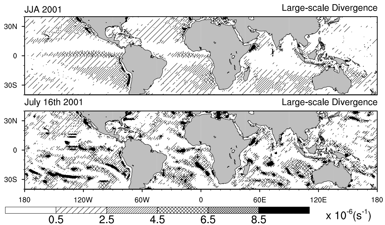
FIG. 10. Large-scale divergence over ocean inferred from ERA-40. Top panel shows the seasonal mean of June, July and August in 2001. Bottom panel shows the daily mean on July 16th, 2001.
