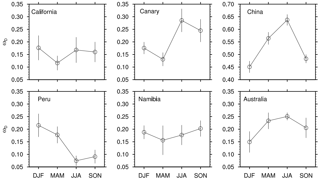
FIG. 17. Seasonal cycle of the occurrence probability of insufficient divergence, \omega_D = \int_{-\infty}^{\mathcal{D}_c} p(\mathcal{D})d\mathcal{D} , based on ERA-40 daily surface divergence data. The circles are the 11-year seasonal mean value while the vertical line denotes interannual standard deviation among 11 years. Please refer to Appendix for details.
