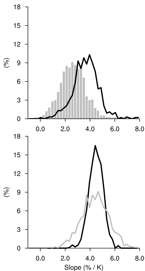
FIG. 16. Top: Distribution of regressions between low-cloud fraction (LCF) and lower-tropospheric stability (LTS) from randomly sampled points from within four of the KH93 stratocumulus regions (Australia, Peru, Californian, Namibian) in Figure 2. Bars show results from the MLM equilibria LCF forced with ERA-40 daily data; the black curve shows the result from sampling the ISCCP data. Four sets of points are drawn from the 12 years within these geographic regions, each set contains approximately the same number of locations as the original regions, producing a set of seasonal averages similar to those in Figure 1 (though without having averaged over multiple years; each seasonal value within the set is drawn from a single year). The bottom panel shows similar distributions based on six sets of points randomly sampled using vertical motion and LTS as selection criteria, LTS > 18.55 K (dark line, corresponds to sampling in the light-shaded region in Figure 2) and LTS > 15 K (light line, corresponds to sampling in the dark-shaded region in Figure 2) based on ERA-40 and ISCCP data. All four distributions are based on 1000 regressions, and binned from -1 to 8 \text{ \% K}^{-1} in 40 intervals.
