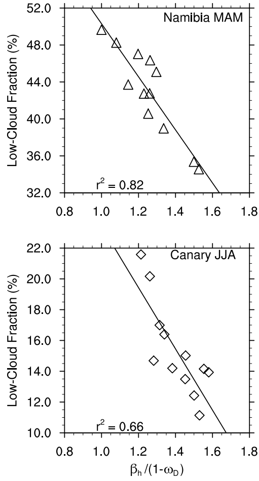
FIG. 18. Least-square regression between low-cloud fraction (LCF) and non-dimensional parameter \beta_h/(1 - \varpi_D) in the season of March, April and May (MAM) at Namibia (top) and the season of June, July and August (JJA) at Canary (bottom). LCF and \beta_h/(1 - \varpi_D) are from MLM equilibrium solutions forced by ERA-40 daily mean data in 12 years (1990 to 2001). \beta_h represents the entrainment exchange velocity normalized by the surface exchange velocity; \varpi_D = \int_{-\infty}^{\mathcal{D}_c} p(\mathcal{D})d\mathcal{D} , is the occurrence probability of insufficient divergence. Please refer to Appendix for details.
