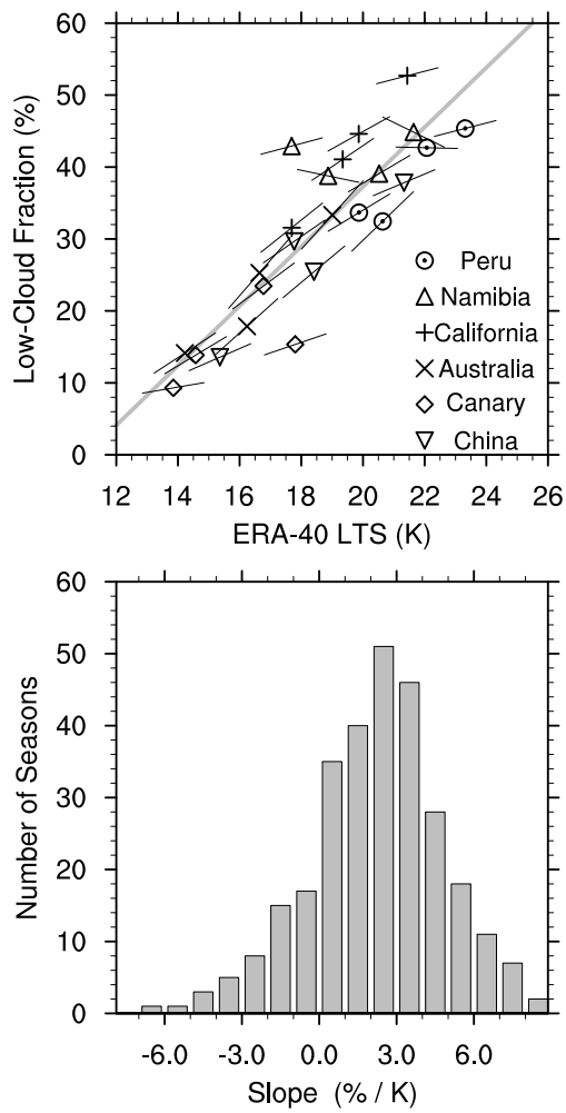
FIG. 15. The emergence of the relationship between low-cloud fraction (LCF) and lower-tropospheric stability (LTS) in different seasons for different regions from the MLM equilibria forced by ERA-40 daily data. Top: The gray line shows the regression between LCF and LTS based on seasonal area-mean values. The black short lines denote the local regression for a particular region and season. Bottom: Histogram of local regression slopes.
