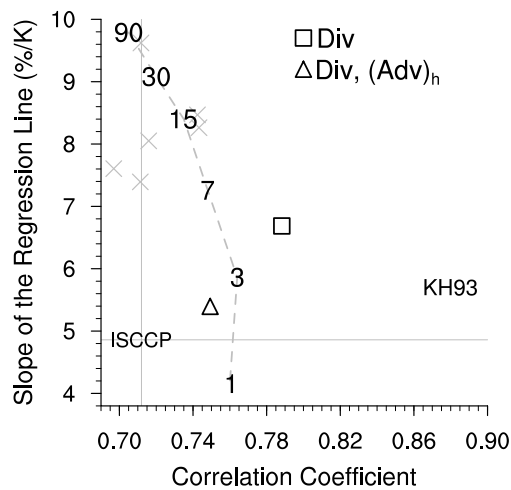
FIG. 9. Transition (gray dashed line) from MLM seasonal (90 days) run to MLM daily (1 day) run in representing the relationship between the MLM equilibrium low-cloud fraction (LCF) and ERA-40 lower-tropospheric stability (LTS): the regression slope (vertical axis) and the correlation coefficient (horizontal axis). Numbers along the dashed line denote the number of days over which daily data is averaged to produce large-scale forcings for the MLM. The intersection of the two gray solid lines, denoted by “ISCCP”, represents the regression between ISCCP LCF and ERA-40 LTS in Figure 1. “KH93” represents the regression from Klein and Hartmann (1993). The gray crosses denote the sensitivity runs in which all the MLM boundary conditions are seasonal averages except one boundary condition, which varies daily; following the order of decreasing regression slope, these crosses are for free troposphere humidity, LTS, free troposphere temperature, surface temperature, horizontal heat and moisture advection, and horizontal mass advection respectively. Specifically the square denotes the sensitivity run with daily varying divergence; the triangle denotes a similar sensitivity run, but with daily forcing for both divergence and horizontal mass advection.
