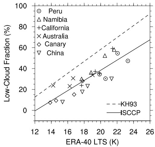
FIG. 1. The least-square regression (solid line) between low-cloud fraction (LCF) from the International Satellite Cloud Climatology Project (ISCCP) and lower-tropospheric stability (LTS) from ECMWF Reanalysis (ERA-40). Different markers denote 12-year (1990-2001) seasonal means in six subtropical regions as shown in Figure 2. The dashed line is the regression between LCF and LTS from Klein and Hartmann (1993).
