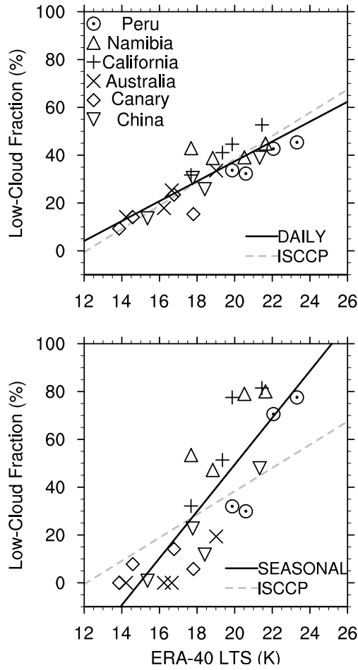
FIG. 8. The least-square regression between seasonal area-mean lower-tropospheric stability (LTS) and low-cloud fraction (LCF) from the MLM equilibria forced by ERA-40 daily data (top) and seasonal averages (bottom). Markers denote different stratocumulus regions in Figure 2. The dashed line is the regression between ISCCP LCF and ERA-40 LTS from Figure 1.
