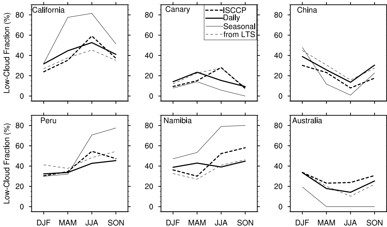
FIG. 6. Seasonal cycles of subtropical low-cloud fraction (LCF) from ISCCP data (dark dashed), MLM daily run (dark solid) and MLM seasonal run (light solid). Light dashed line denotes the LCF diagnosed from lower-tropospheric stability (LTS) based on the regression between ISCCP LCF and ERA-40 LTS in Figure 1.
