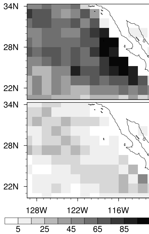
FIG. 5. Low-cloud fraction (in percent) offshore of southern California, July 2001 from MLM equilibrium simulation forced by ERA-40 daily mean data. The top panel shows the results with cloudy initial states while the bottom one shows the difference (decrease) if using clear-sky initial states.
