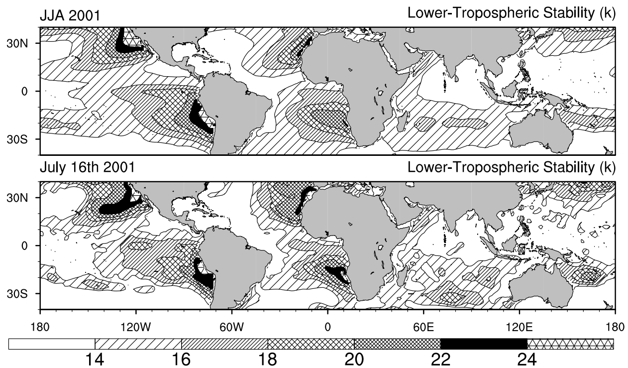
FIG. 11. Same as in Figure 10 but for lower-tropospheric stability over ocean.
