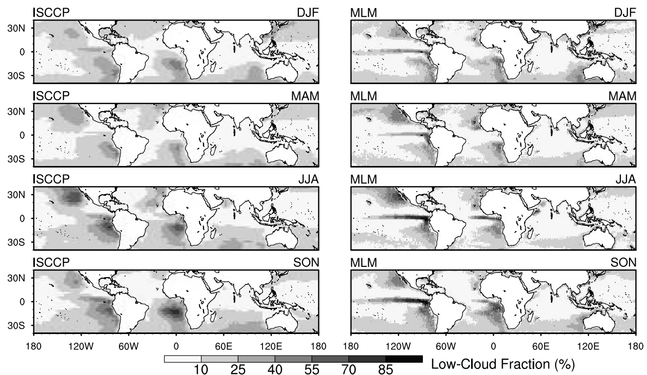
FIG. 7. Seasonal mean low-cloud fraction measured by ISCCP (left) and indicated from the mixed-layer model equilibria with ERA-40 daily forcing (right) over ocean averaged in 12 years (1990-2001).
